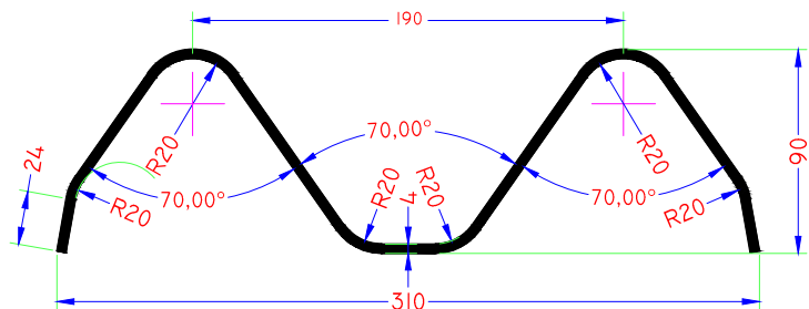
FINAL PROFILE OF ROAD GUARD - 492 MM SHEET WIDTH
